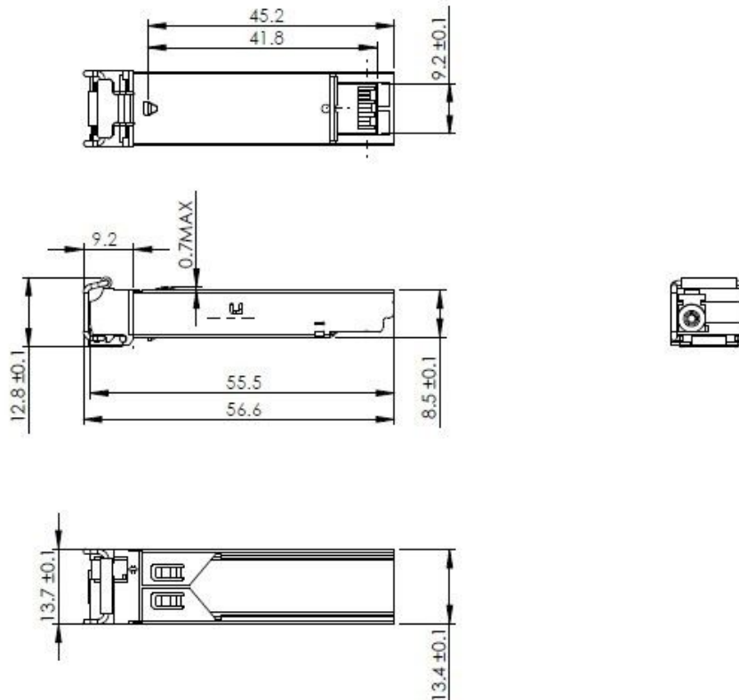
Mechanical Drawing
