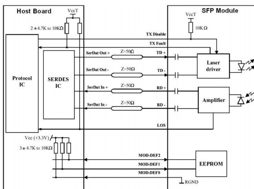
SFP Host Recommended Circuit
