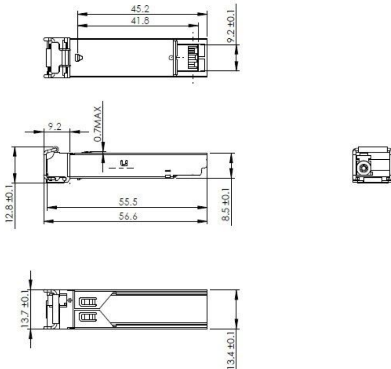
Mechanical Drawing
