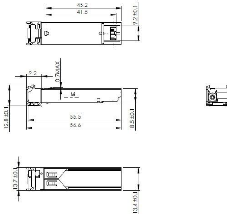
Mechanical Drawing
