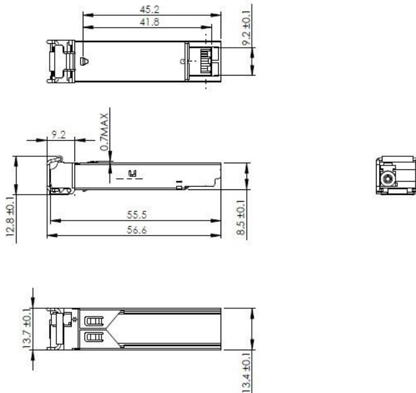
Mechanical Drawing
