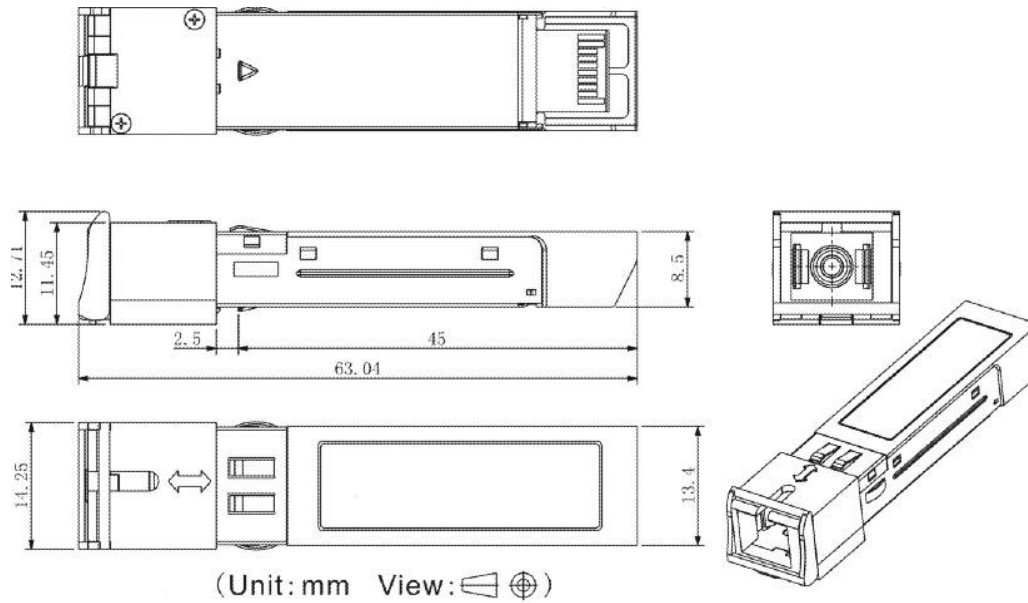
Mechanical Drawing
