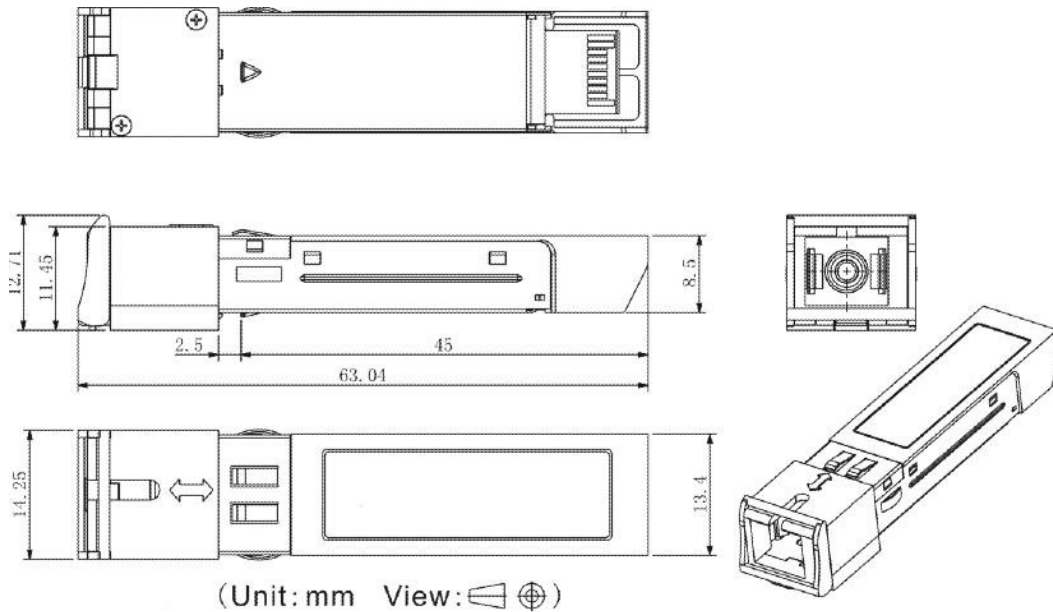
Mechanical Drawing
