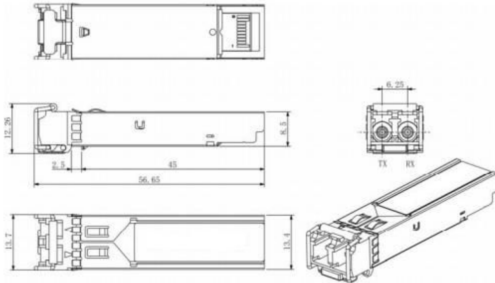
Mechanical Drawing
