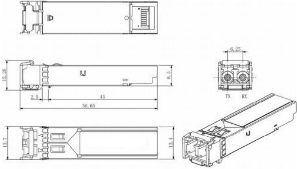
Mechanical Drawing
