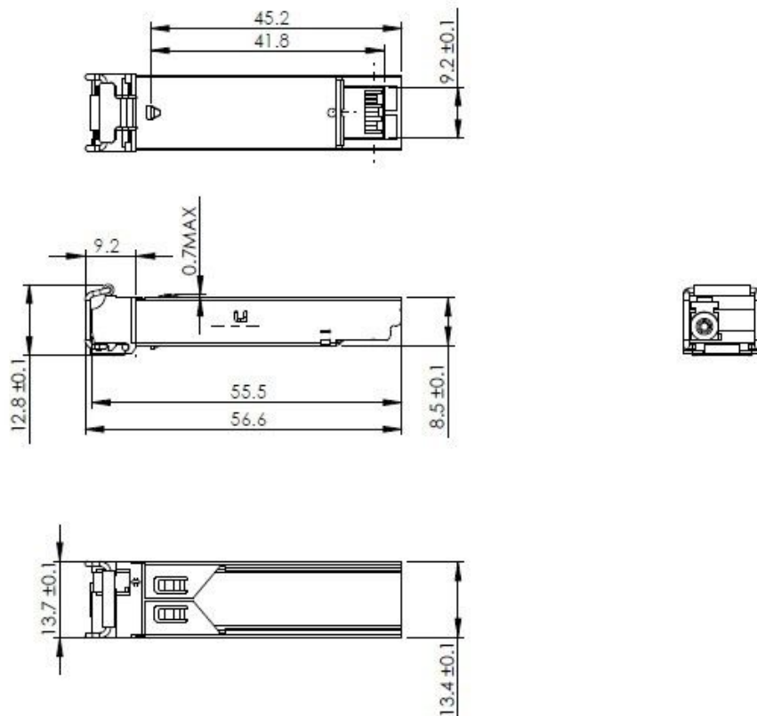
Mechanical Drawing
