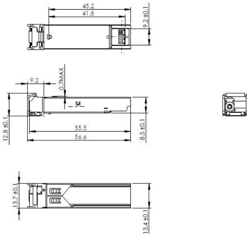
Mechanical Drawing
