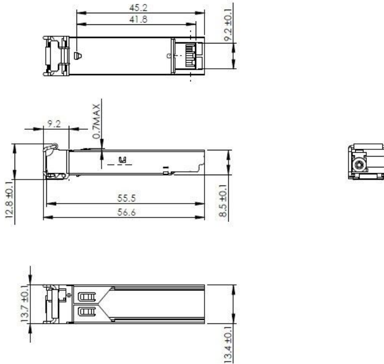
Mechanical Drawing
