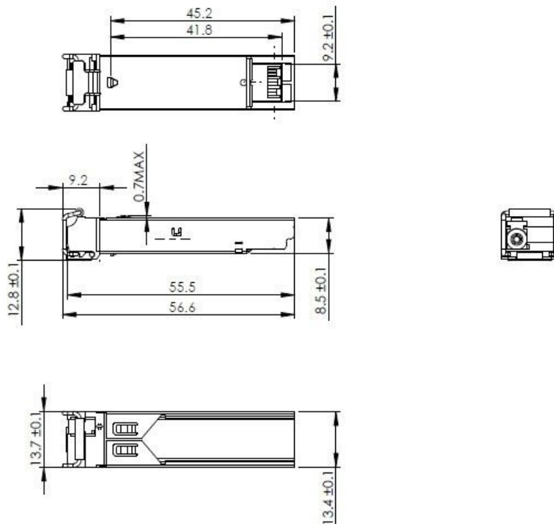
Mechanical Drawing
