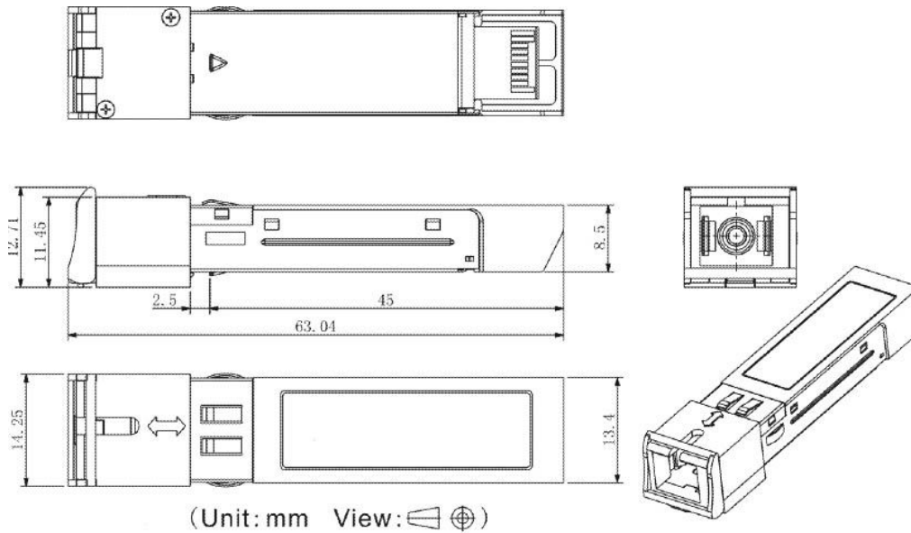
Mechanical Drawing
