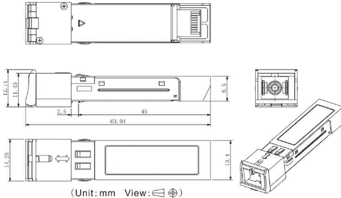
Mechanical Drawing
