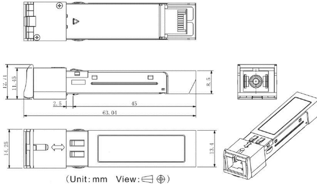
Mechanical Drawing
