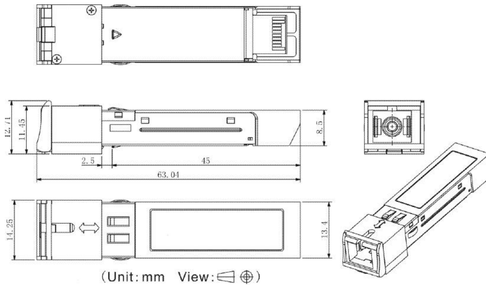
Mechanical Drawing
