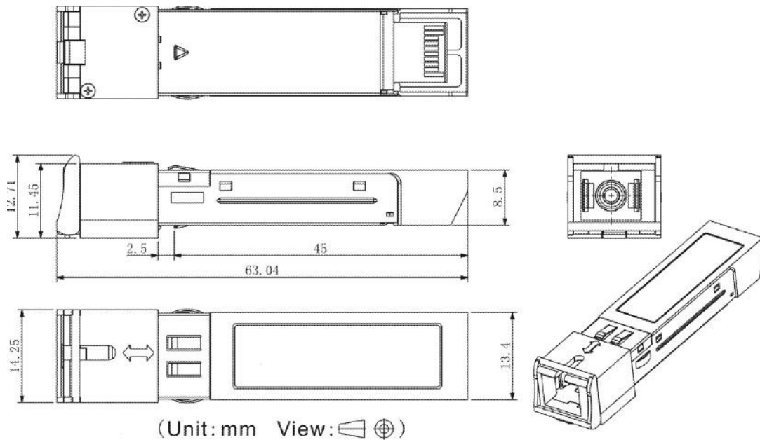
Mechanical Drawing
