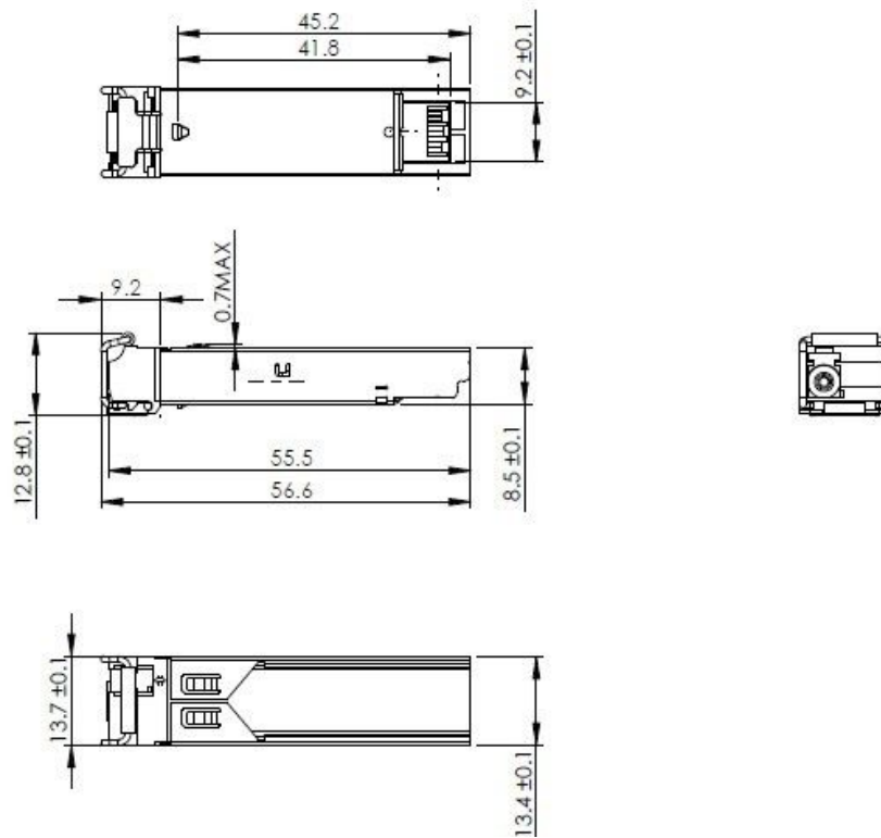
Mechanical Drawing
