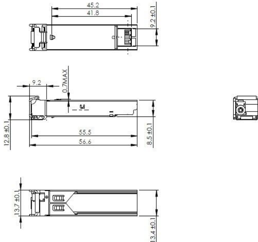
Mechanical Drawing
