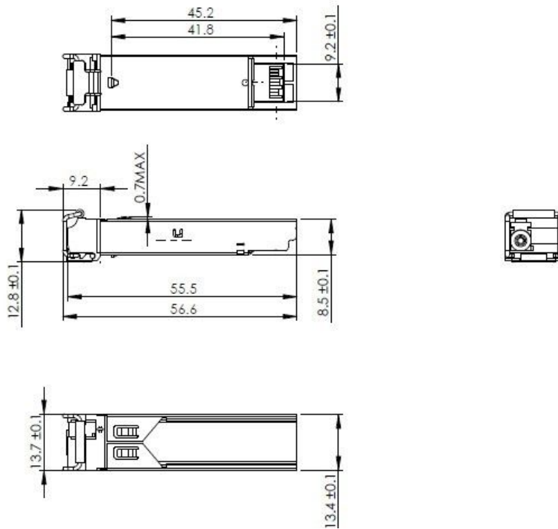
Mechanical Drawing
