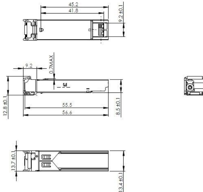
Mechanical Drawing
