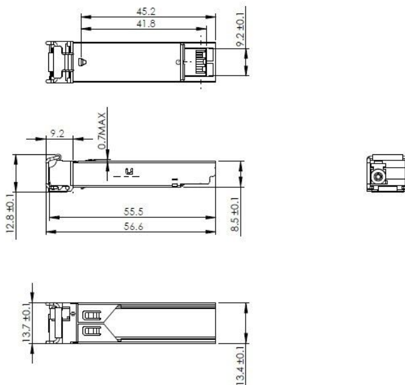
Mechanical Drawing
