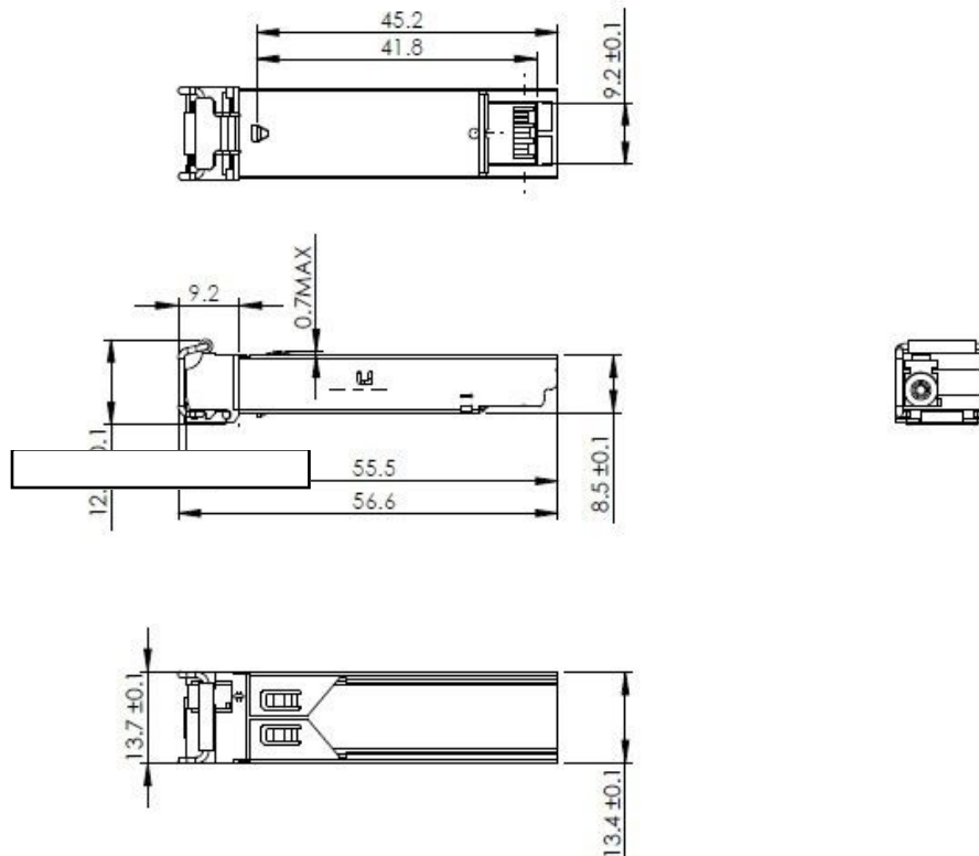
Mechanical Drawing
