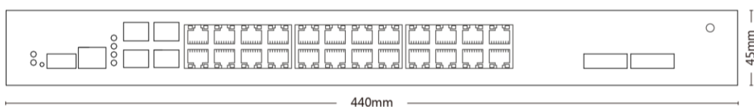
Front view
